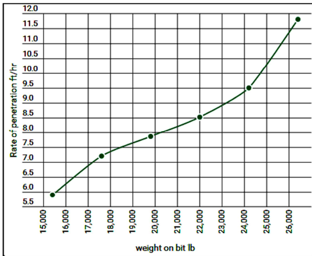
Figure 3. The Effect Of Bit Loading at depth 4216.06 ft.
